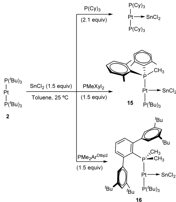
Scheme 5 Tin-mediated phosphine exchange reactions at Pt(0) 2.
