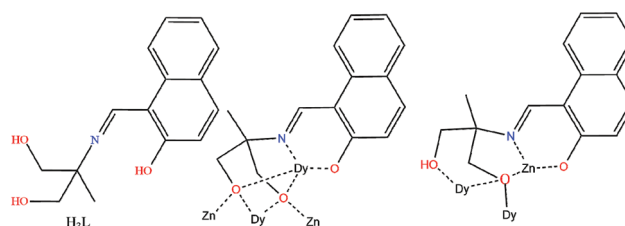
Scheme 1 The ligand and its coordination modes in 1.
