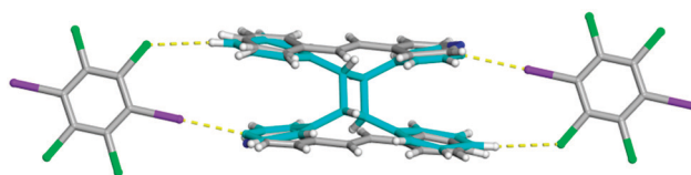
Fig. 4 X-ray structure of the partially photoreacted co-crystal of form I forming the ht -PP shown in turquoise. The I\cdots N halogen bonds and C-H \cdots Cl contacts are shown with yellow dashed lines.
