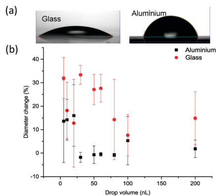
Fig. 4 (a) Lateral images of a drop of water on glass and aluminium foil substrates and (b) change of the diameter up to the start of crystallisation of printed drops as a function of drop size.
