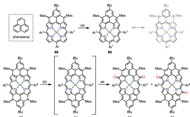
Fig. 30 Peripherally phenalenyl-fused porphyrins. Reagents and conditions: (a) 2 equiv. NIS, \text{CH}_2\text{Cl}_2 , rt, 5 min, 49%; (b) 2 equiv. p -chloranil, \text{CH}_2\text{Cl}_2 , rt, 10 min. 92 and 93 were obtained after exposure to air for 3.5 h, 20% for 92 , 39% for 93 . \text{Ar}^1 = 4 - tert -butylphenyl, \text{Ar}^2 = 3,5 -di- tert -butylphenyl.
