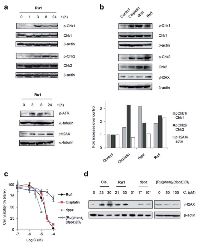
Fig. 2 (a) DNA damage response (DDR) activation by Ru1 . Whole-cell extracts of OE21 cells treated with Ru1 (20 μM) for 1, 3, 8 or 24 h were immunoblotted for activated (phosphorylated, p-) p-Chk1 (Ser345), p-Chk2 (Thr68), p-ATR (Ser428) or γH2AX (pH2AX at Ser139), as indicated. Total Chk1 and Chk2 protein levels independent of phosphorylation status are shown. α-Tubulin or β-actin were used as loading controls. (b) Relative expression of pChk1 and pChk2 in OE21 cells treated with equipotent (IC 50 ) concentrations of cisplatin (23 μM), dppz (7 μM) or Ru1 (21 μM) for 3 h, as determined by immunoblotting and quantified by densitometry (bottom panels). Phosphorylated protein levels relative to total protein and normalised to control are presented. γH2AX/β-actin ratio also provided. (c) Impact of Ru1 , dppz, [Ru(phen) 2 (dppz)] 2+ or cisplatin on viability of OE21 cells, as determined by MTT assay (24 h incubation time). Mean of quadruplicates ± S.D. and representative of two independent experiments. (d) Immunoblotting of γH2AX levels in OE21 cells after 24 h treatment with cisplatin (Cis), Ru1 or dppz (IC 50 and IC 70 concentrations). [Ru(phen) 2 (dppz)] 2+ treatment also included. β-Actin was used as a loading control. * 0.25% DMSO.
