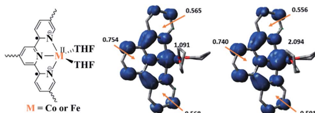
Fig. 7 Proposed electronic structure of M II (THF) 2 ·(TPY •• ) 2- -MOL, M = Co or Fe (left); calculated Mulliken spin density distribution and spin density plots (blue: positive; green: negative) of Co(tpy)(THF) 2 quartet state (middle) and Fe(tpy)(THF) 2 quintet state (right).
