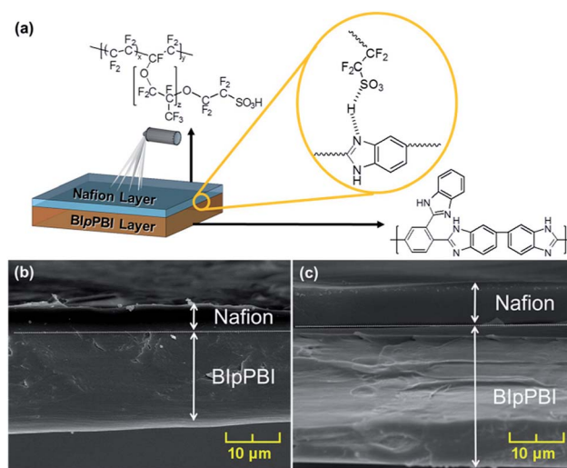
Fig. 1 (a) Schematic of the BI l PBI/Nafion hybrid membrane and its interface; cross sectional SEM image of (b) B20N5 and (c) B20N10.
