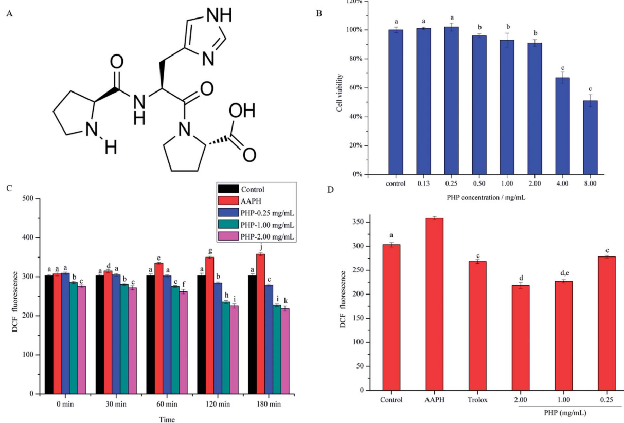
Fig. 1 The chemical structure of the tripeptide, Pro-His-Pro (PHP) (A). Effects of PHP on the viability of HepG2 cells (B). Intracellular ROS scavenging capacities of different concentrations of PHP and different incubation time under conditions of AAPH-induced oxidative stress in HepG2 cells (C). Intracellular ROS scavenging capacities of different concentrations of PHP and Trolox at 180 min of incubation (D). Data are presented as the mean \pm SD. Different letters indicate significant differences at P < 0.05 , n = 3 data points.
