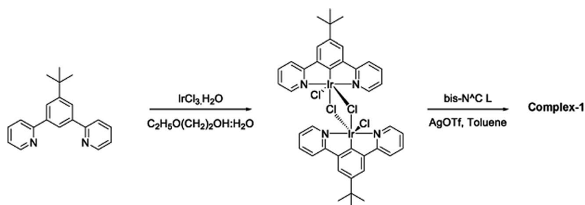
Fig. 3 Synthesis of [(N^{\wedge}C^{\wedge}N)_2Ir(bis-N^{\wedge}C^{\wedge}N)Ir(N^{\wedge}C^{\wedge}N)_2Cl]PF_6 ( N^{\wedge}C^{\wedge}N = 2-[3- tert -butyl-5-(pyridin-2-yl)phenyl]pyridine; bis- N^{\wedge}C^{\wedge}N = 3,6-bis(4- tert -butylphenyl)pyridazine) (complex-1) by reaction of dichloro-bridged iridium(III) dimer with the bis-bidentate proligand in toluene, using silver triflate as a chloride scavenger.
