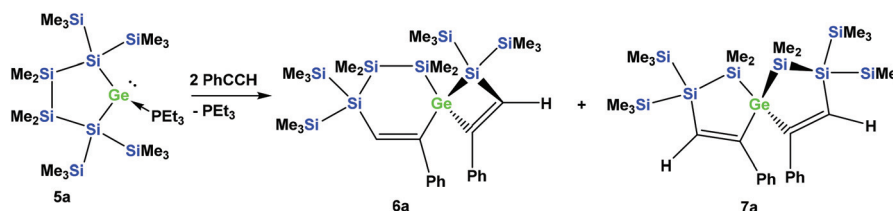
Scheme 2 Reaction of cyclic digermylene phosphane adduct 5a with phenylacetylene.
