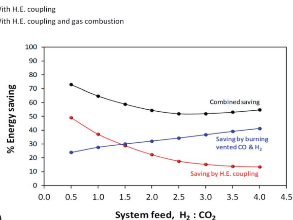
Fig. 8 Efficiencies for the methanol synthesis system for two extreme cases: (a) a \text{H}_2 -CO only feed and (b) a \text{H}_2 -CO 2 only feed. The 'no losses' scenario is a theoretical-only case in which the syngas conversion process consumes no energy and vented gases do not constitute energy loss. The corresponding energy savings made by coupling heat exchangers and by combustion of vented gases are shown in (c) and (d).
