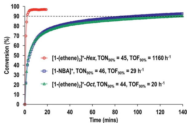
Fig. 9 Comparison of SMOM-cat in the isomerization of 1-butene to 2-butene as measured by gas phase 1 H NMR spectroscopy. All catalysts = ~2.5 mg sample (~1.7 μmol). 1-Butene = 1 atm (86 μmol at 298 K). Dashed line indicates 90% conversion.
