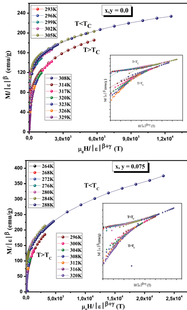
Fig. 12 Scaling plots for \text{La}_{0.7}\text{Ca}_{0.1}\text{Pb}_{0.2}\text{Mn}_{1-x-y}\text{Al}_x\text{Sn}_{1-y}\text{O}_3 ( x, y = 0.0 and 0.075 ) below and above T_c using \beta and \gamma determined by the Kouvel–Fisher method. The insets show the same plots on a log–log scale.
