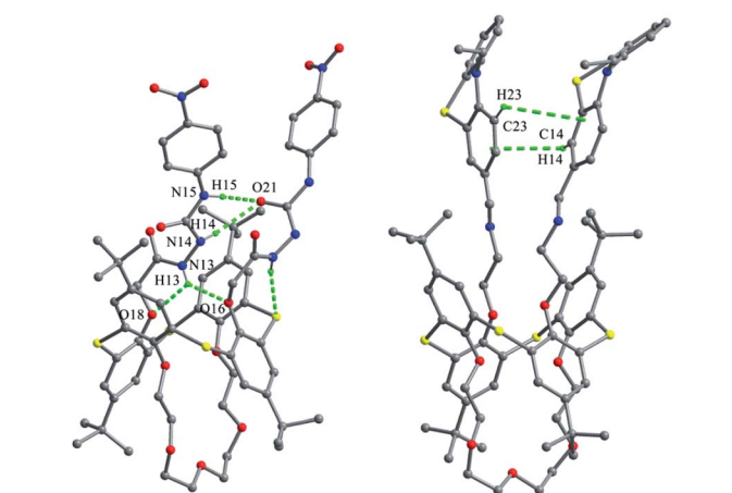
Fig. 70 Crystal structures of 74 (left) showing H-bonds, and 75 (right) showing C-H... \pi contacts.
