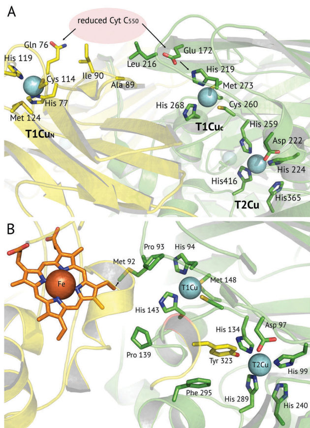
Fig. 6 Proposed electron transfer routes between the redox centres of 3-domain CuNiRs. In (A) HcNiR the external electron donor partner protein cyt. c 550 is proposed to bind to a hydrophobic patch spanning the N-terminal (near Ala89, Ile90) and cupredoxin domains (near Leu216), where it is positioned for electron transfer to both the T1Cu N and T1Cu C sites (indicated by arrows). 74 In (B) RpNiR , the proposed internal electron transfer route is from the haem (CBC atom) to Met92 and to the T1Cu site. 75 Interface and T2Cu water molecules have been omitted from the figures for clarity.
