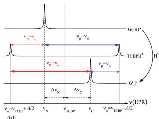
Scheme 1 Schematic representation of triplet-singlet interconversion based on the EPR spectra of G(H) \cdot (top), TCBPH \cdot (middle), and (G \cdot )' (bottom). Only a single spin-1/2 nucleus in TCBPH \cdot with negative HFCC is considered.
