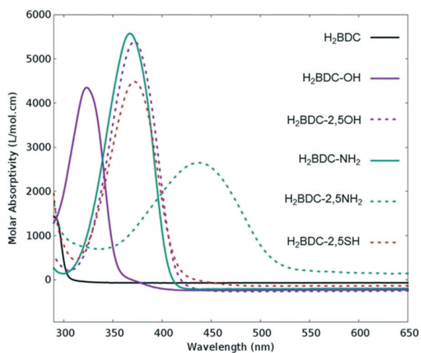
Fig. 1 Experimental UV/VIS absorption spectra of different ligands used for the synthesis of UiO-66 frameworks for photocatalysis. Adapted with permission from ref. 41. Copyright 2015 American Chemical Society.
