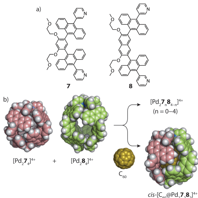
Fig. 6 (a) Short (7) and long (8) anthracene-functionalized ligands; (b) C_{60} -templated integrative self-sorting of cages [Pd_27_4]^{4+} and [Pd_28_4]^{4+} to give the heteroleptic host-guest complex cis-[C_{60}@Pd_27_28_2]^{4+} . Reproduced with permission from ref. 54.
