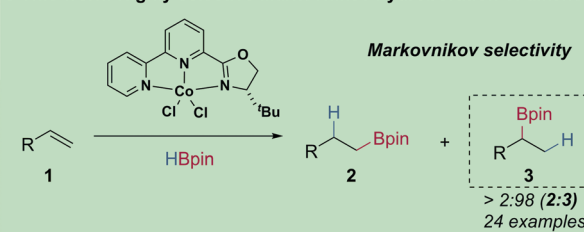
Scheme 1 (A) Anti-Markovnikov selective cobalt-catalysed alkene hydroboration. (B) Markovnikov selective cobalt-catalysed hydroboration of alkenes. (C) This work: t BuBPOCoCl 2 -catalysed highly selective Markovnikov hydroboration of alkenes.
