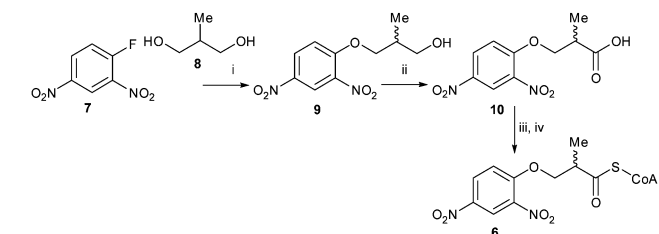
Scheme 2 Synthesis of substrate 6. Reagents & conditions: (i) Na metal, 83%; (ii) CrO 3 , conc. H 2 SO 4 , acetone, 67%; (iii) carbonyldiimidazole, CH 2 Cl 2 ; (iv) CoA-SH (Li + ), 0.1 M NaHCO 3 aq/THF (1:1).
