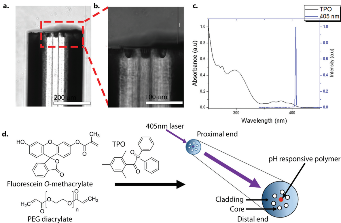
Fig. 1 (a)–(b) Lateral images of an etched optical fibre. The depth of a pit was approximately 30 \mu\text{m} . The distal end of the optical fibre was HF-etched and silanized in 3-(trimethoxysilyl)propyl methacrylate (TMSPMA) (20 v/v% in acetone) to introduce acrylate groups onto the distal surface of the pit. Scale bar (a) = 200 \mu\text{m} and scale bar (b) = 100 \mu\text{m} . (c) The absorbance spectrum of diphenyl(2,4,6-trimethylbenzoyl)phosphine oxide (TPO) (2.5 mM in ethanol) (black line), and the 405 nm laser spectrum (blue line). TPO absorbs in the UV range up to about 425 nm, and although not optimal, it allowed sufficient excitation and radical generation by TPO (it is worth noting that the light source used by dentists with this initiator are typically in the wavelength range of circa 380 to 520 nm (dual peak LED)). 23 (d) The method used for photo-polymerisation at the distal end of the optical fibre. Only seven (of the 19) cores of the optical fibre are shown for clarity. The laser was coupled to a specific core of the fibre via an XYZ translation stage. Once coupled, the distal end was dipped into the polymerisation solution containing fluorescein O -methacrylate 0.17 M, PEG-diacrylate 1.37 M and TPO 0.05 M.
