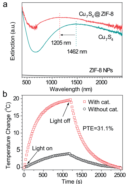
Fig. 2 (a) Extinction spectra of \text{Cu}_7\text{S}_4 , ZIF-8, and \text{Cu}_7\text{S}_4 @ZIF-8 NPs. The spectra were collected by dispersing the samples in a KBr matrix. (b) Steady state heating data (bulk temperature) of the dichloromethane solution with or without the \text{Cu}_7\text{S}_4 @ZIF-8 NPs irradiated by a 1450 nm laser light with an intensity of 500 \text{ mW cm}^{-2} .
