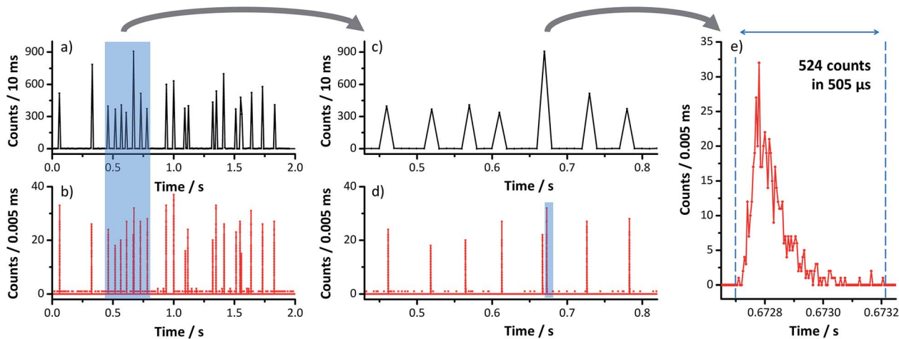
Fig. 1 Representative ICP-MS signal (monitoring m/z^{197}\text{Au} ) due to 30 nm AuNPs ( C_{\text{NP}} = 2.5 \times 10^5 \text{ NP mL}^{-1} ) acquired simultaneously for 2 s with (a) 10 ms dwell time (vendor software), and (b) 5 \mu\text{s} dwell time (home-built DAQ). First zoom level shows several particle events in (c) and (d) for 500 ms (of highlighted section in a and b). Second zoom level (e) shows the temporal profile of a single particle's ion cloud identified with the home-built DAQ in (d).
