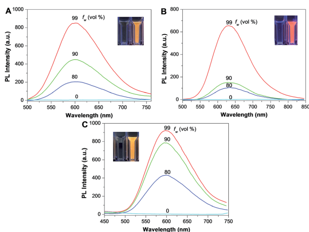
Fig. 2 Fluorescence spectra of TPDC (A), TPDCP (B), PPDC (C) in DMSO/water mixtures with different volume fractions of water at a concentration of 10 \mu M. The excitation wavelengths for (A), (B) and (C) are 400, 390, 420 nm, respectively. The insets show photographs of the compounds in DMSO and DMSO : water ( v/v, 1:99 ) under UV light (365 nm) illumination.
