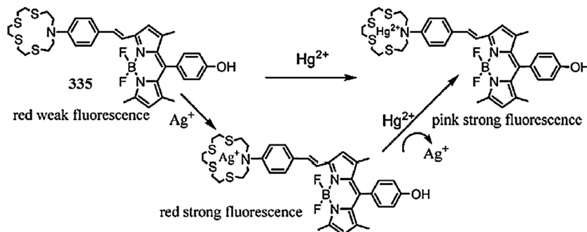
Fig. 295 Proposed binding mechanism of probe 335 toward Hg 2+ and Ag + .
