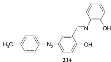
Fig. 179 Chemical structure of 2-[(2-hydroxy-1-propenyl-but-1,3-dienylimino)-methyl]-4- p -tolylazo-phenol 214 .
