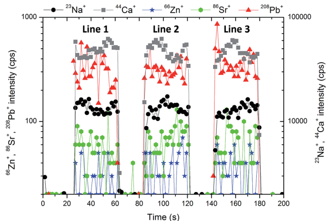
Fig. 2 The stability of the signal of ^{23}\text{Na}^+ , ^{44}\text{Ca}^+ , ^{66}\text{Zn}^+ , ^{86}\text{Sr}^+ , ^{208}\text{Pb}^+ during the ablation of pellet no. 7851 within 3 lines with the length of 1.5 mm, approximately.
