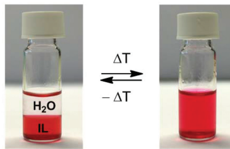
Fig. 8 Reversible formation of a homogeneous phase when increasing the temperature above the cloud point ( 55^\circ\text{C} for a pure water/ionic liquid system in a 1 : 1 ratio). 44 A coloring agent (methyl red sodium salt) was dissolved in the transparent ionic liquid phase to help the visualization. The density of the [Hbet][Tf_2N] liquid is higher than that of water.
