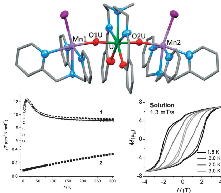
Fig. 17 (top) Molecular structure of \{[M(\text{TPA})][\text{UO}_2(\text{Mesaladien})][M(\text{TPA})]\} ( M = \text{Mn} ( \text{Mn}_2\text{U} ), \text{Cd} ( \text{Cd}_2\text{U} )) with hydrogen atoms omitted for clarity; (bottom left) Susceptibility temperature product as a function of temperature for \text{Mn}_2\text{U} (1) and \text{Cd}_2\text{U} (2), as well as their difference (open symbols), showing the effective ferromagnetic coupling between \text{U}^{\text{V}}\text{O}_2 and \text{Mn}^{\text{II}} . (bottom right) Magnetic hysteresis recorded on a pyridine solution of \text{Mn}_2\text{U} . Adapted with permission from ref. 54. Copyright 2014 Wiley-VCH.
