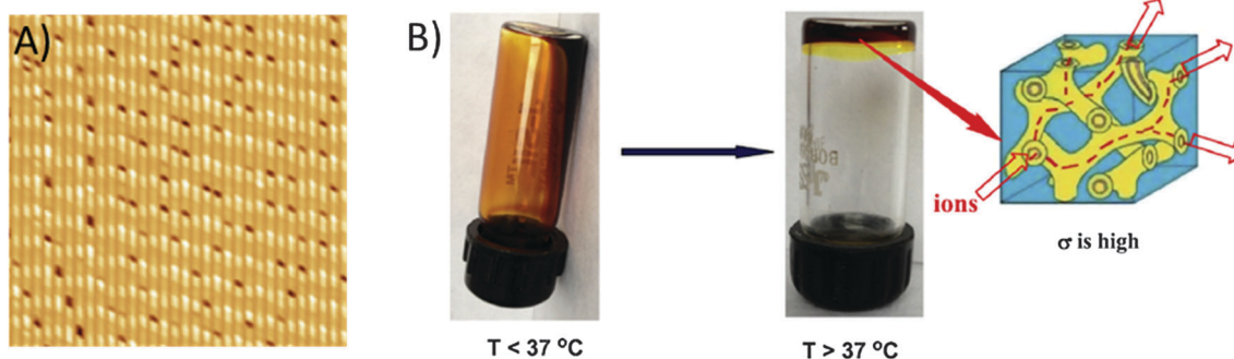
Fig. 24 (A) AFM image of a F77-based gel-polymer electrolyte coated onto a glass substrate. Black dark spots prove the existence of a circular area ranging from 3 to 5 nm, which might be the core of F77 micelles consisting of hydrophobic PPO moieties. The contrast of this area to the rest of the film could be due to the penetration of relatively hydrophobic I 3 - into the PPO core. (B) Photos and schematic illustration of the structural polymorphism of a F77-based gel-polymer electrolyte. Adapted and reprinted from ref. 314.
