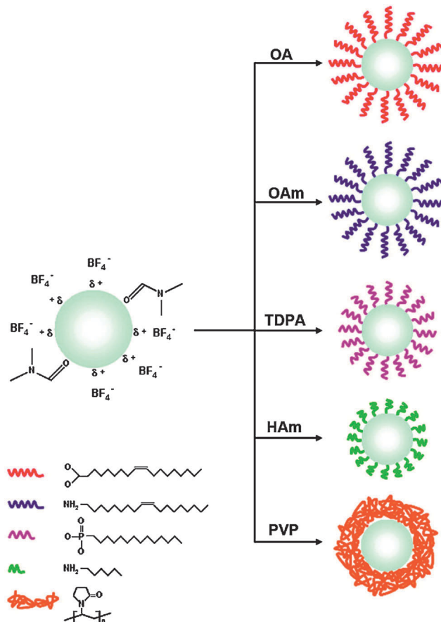
Fig. 8 Subsequent ligand exchange reactions of \text{BF}_4^- -coated UCNP in dimethylformamide (DMF). The use of oleic acid (OA), oleylamine (OAm), tetradecylphosphonic acid (TDPA), or hexylamine (HAm) yields hydrophobic UCNP dispersible in hexane, while the use of polyvinylpyrrolidone (PVP) results in UCNP dispersible in aqueous media. Adapted with permission from ref. 135. Copyright © 2011, American Chemical Society.
