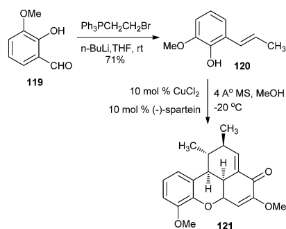
Scheme 27 Synthesis of benzoxanthrone 121 .
