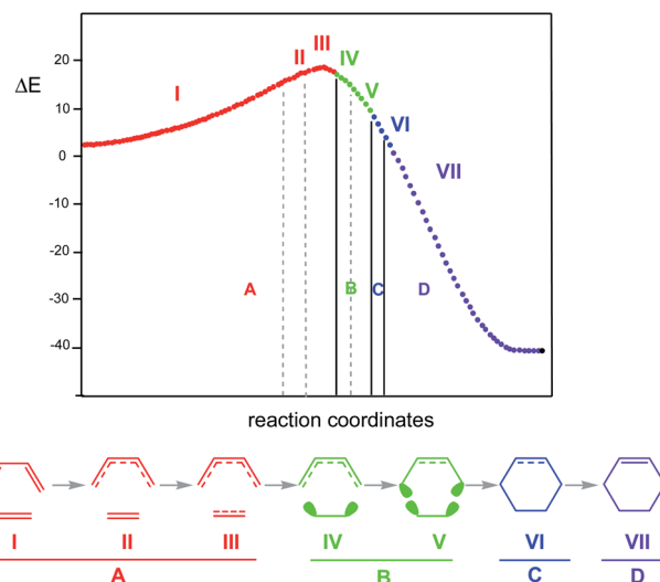
Fig. 6 Reaction path calculated by means of the IRC method for the DA reaction between butadiene 1 and ethylene 2 . \Delta E are in \text{kcal mol}^{-1} . A bonding between atoms in all phases is demonstrated by the standard Lewis representation; however, in the case of phases IV and V, ellipses reflect the non-bonding electron density concentrated in the C atoms. The four colours represent the four main groups in which the bonding changes can be categorised.
