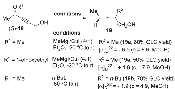
Scheme 5 Synthesis of optically active 2-substituted \alpha -allenols via chirality transfer.
