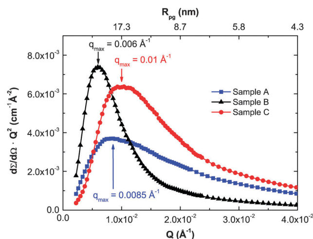
Fig. 2 Kratky plot of the SANS curves. Each curve exhibits a broad maximum, which yields the pseudo-Guinier radius R_{\text{pg}} .
