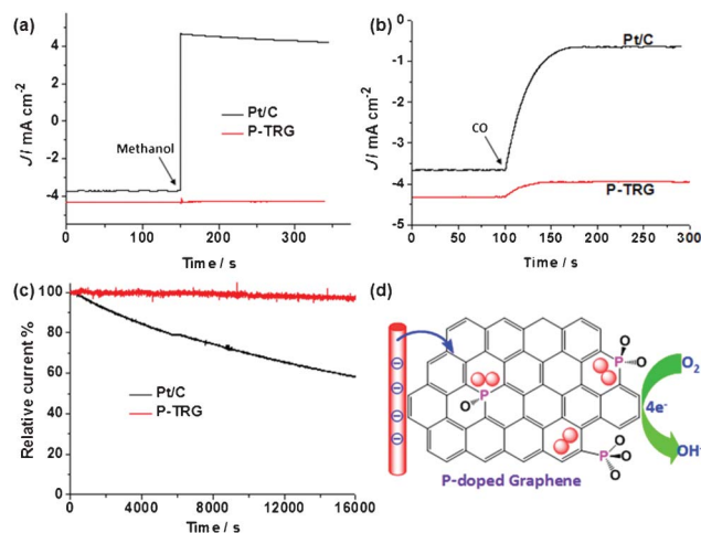
Fig. 5 (a) Methanol crossover tests by injecting methanol into the electrolyte at 150 s to make the final concentration of methanol 3.0 M. (b) CO poisoning tests by introducing additional CO with the same flow of O_2 into the electrolyte from 100 s. (c) Comparison of the stability of the P-TRG and Pt/C electrode at -0.26 V in O_2 -saturated 0.1 M KOH solution at a rotation rate of 1600 rpm. (d) Schematic illustration of the possible ORR process catalyzed by the P-doped graphene.
