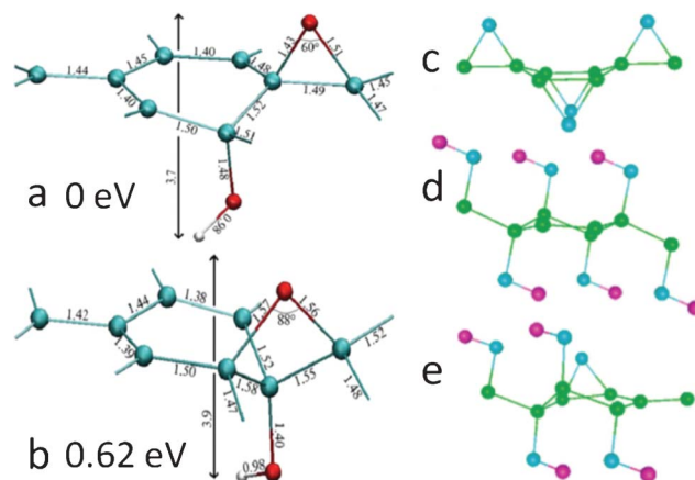
Fig. 4 (a) and (b): detailed geometric configurations of GO with one ether and one hydroxyl in a unit cell with eight carbon atoms. The interatomic distances are in angstrom. Carbon, oxygen, and hydrogen atoms are shown in green, red, and white, respectively. (a) and (b) have 1,2-ether and 1,3-ether oxygens, respectively. Reprinted with permission from ref. 114. Copyright (2009) by the American Physical Society. (c)–(e): the most stable structures of GO with only epoxies (c), hydroxyls (d), and mixed coverage (e). Carbon, oxygen, and hydrogen atoms are shown in green, blue, and violet, respectively. Reprinted with permission from ref. 99. Copyright (2008) American Chemical Society.
