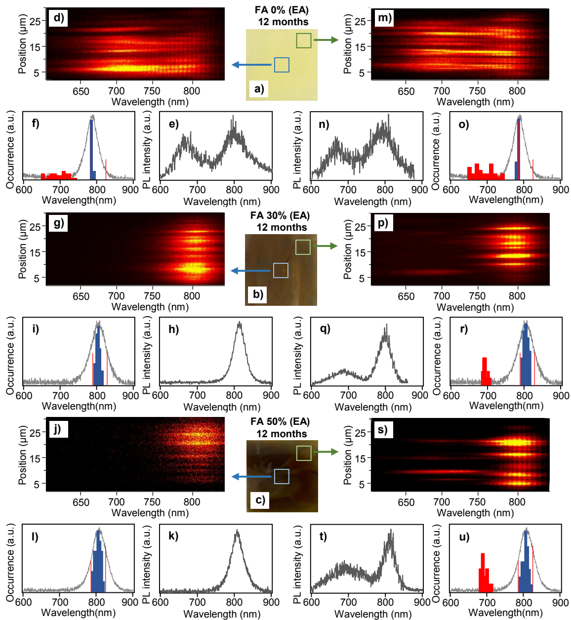
Figure 2. Spectroscopic characterization of the degradation process. (a)-(c) Photographs of perovskite films of different compositions as indicated in the figure taken 12 months after the films fabrication. The squares and arrows indicate symbolically the areas used for the spectral measurements. (d), (g), (j) Representative 2D PL spectral plots (position vs. wavelength) for central locations in the respective films. (m), (p), (s) Same plots for locations close to the film edges. (e), (h), (k) Examples of typical PL spectra taken in central locations
