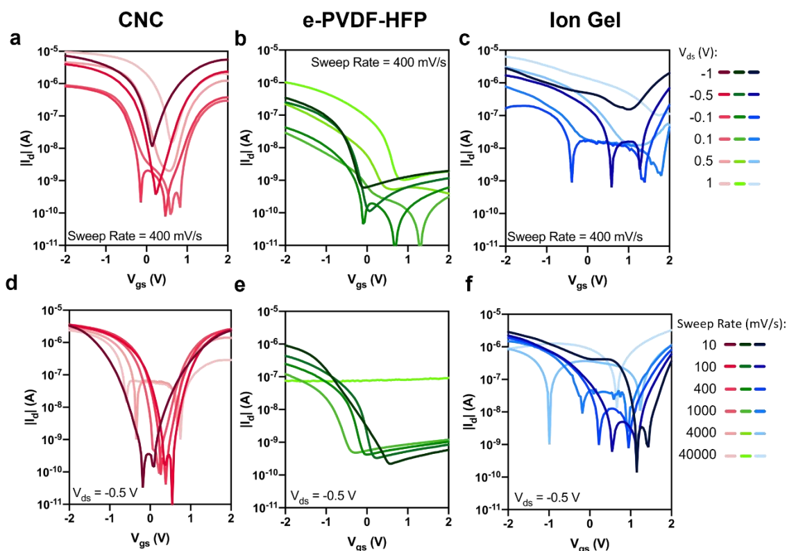
Figure 4. Dependence of CNT-TFT performance on drain-source voltage and gate sweep rate. V_{ds} dependence with a fixed sweep rate of 400 mV/s for (a) CNC, (b) e-PVDF-HFP, and (c) ion gel, revealing reasonably consistent switching for the CNC and e-PVDF-HFP devices up to |1\text{ V}| and degradation for the ion gel device above |0.5\text{ V}| . Sweep rate dependence with a fixed V_{ds} = -0.5\text{ V} for (d) CNC, (e) e-PVDF-HFP, and (f) ion gel, showing robust switching for the CNC up to 4 V/s and complete loss of switching behaviour in the e-PVDF-HFP above 1 V/s. For all devices, L_{ch} = 250\text{ }\mu\text{m} and W_{ch} = 200\text{ }\mu\text{m} .
