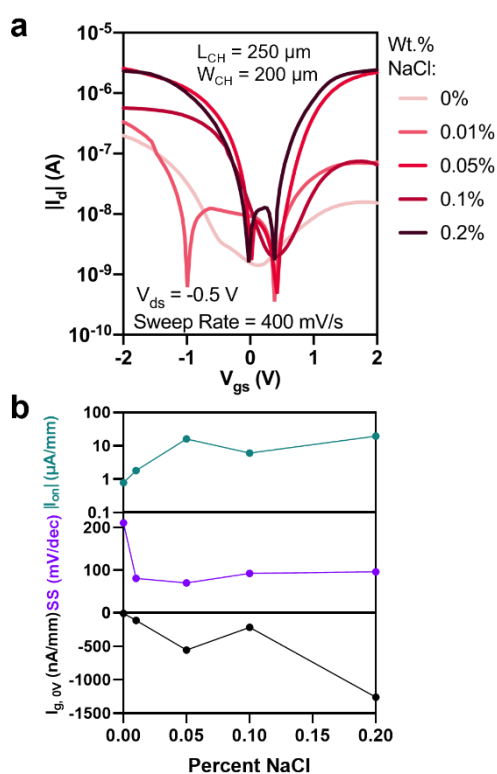
Figure 2. Optimization of CNC salt concentration. (a) Subthreshold curves of printed CNT-TFTs using CNC with salt (NaCl) concentration ranging from 0 – 0.2%. (b) Percent NaCl dependence curves for on-current, subthreshold swing, and gate leakage current at a gate voltage of 0V, revealing a trade-off between high on-current and unwanted gate leakage with increasing salt concentration.
