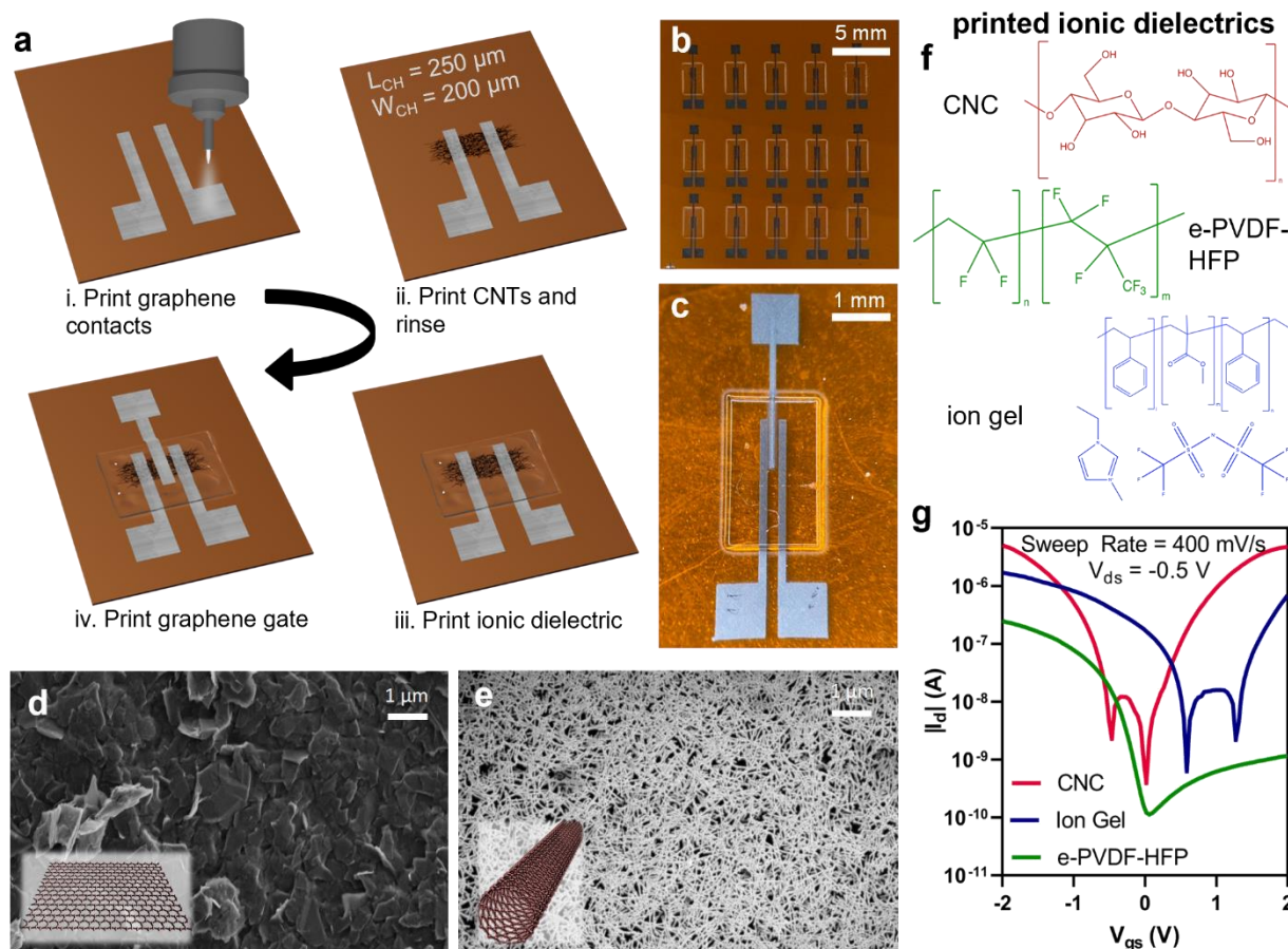
Figure 1. Process flow and structure for fully printed, top-gated CNT-TFTs. (a) Fabrication of devices included: (i) Printing graphene source and drain contacts on KOH-treated Kapton, (ii) CNT film printing then rinsing with toluene, (iii) printing of ionic dielectric layer, and (iv) printing of graphene gate contact over dielectric layer, completing the device. Images of (b) array of printed CNT-TFTs with 0.05% CNC as the dielectric and (c) one printed CNT-TFT with ion gel as the dielectric. SEM images of (d) graphene and (e) semiconducting carbon nanotubes showing thin-film morphology when printed on SiO 2 with insets of their respective chemical structures. Note, all printing carried out with an aerosol jet printer using ultrasonic aerosolization. (f) Chemical structures of CNC, e-PVDF-HFP, and ion gel. (g) Subthreshold curves for example CNT-TFTs using CNC, e-PVDF-HFP, or ion gel. For all devices, L_{CH} = 250 \mu\text{m} and W_{CH} = 200 \mu\text{m} .
