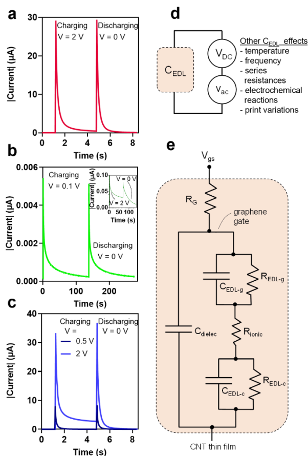
Figure 3. Capacitance characterization for each dielectric. Charging and discharging currents as a function of time for (a) CNC, (b) e-PVDF-HFP with an inset showing charging current at an applied voltage of 2 V, and (c) ion gel. Top and bottom electrode of the capacitors have dimensions of 2.3 mm x 1.5 mm. (d) Representative schematic of the capacitor measurement setup with applied DC and AC voltages and a list of external factors that influence the measurements. (e) Simplified equivalent circuit between the graphene gate and the CNT channel. V_{gs} , R_G , C_{dielec} , C_{EDL-g} , R_{EDL-g} , R_{EDL-c} , C_{EDL-c} , and R_{ionic} stand for the gate voltage, the series resistance of the graphene gate, the dielectric capacitance, the electric double layer capacitance at the graphene/dielectric interface, the resistance corresponding to the (electrochemically originated) leakage at the graphene/dielectric interface, the electric double layer capacitance at the CNT/dielectric interface, the resistance corresponding to the leakage at the CNT/dielectric interface, and ionic resistance, respectively.
