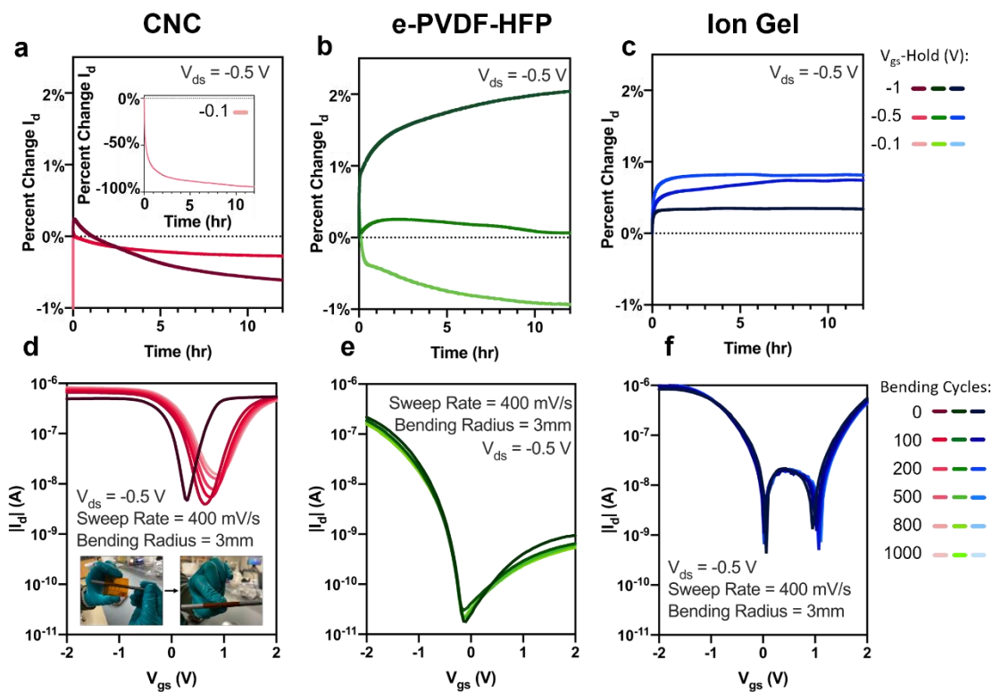
Figure 5. Electrical and mechanical stress tests. Percent change over 12 hours of gate-source voltage bias for (a) CNC, (b) e-PVDF-HFP, and (c) ion gel. Subthreshold curves of bending cycles from 0 to 1000 cycles for (d) CNC with inset image before and during bending, (e) e-PVDF-HFP, and (f) ion gel. For all devices, L_{ch} = 250 \mu\text{m} and W_{ch} = 200 \mu\text{m} .
