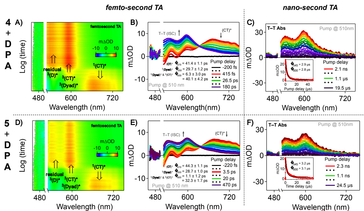
Fig. 7. Time-resolved transient absorption 2D intensity map/spectra for dyads 4 and 5 in the presence of free DPA in oxygen-free THF. (A & B) fs-TA map/spectra for 4 + DPA and (D & E) fs-TA map/spectra for 5 + DPA . Sample O.D. = 0.4 at \lambda_{Exc} = 510 nm. Pump power = 0.3 μJ/pulse and 2.5 kHz repetition rate for fs-TA and 1 μJ/pulse and 1 kHz repetition rate for ns-TA. The molar ratio of Dyad:DPA is 1:3.
