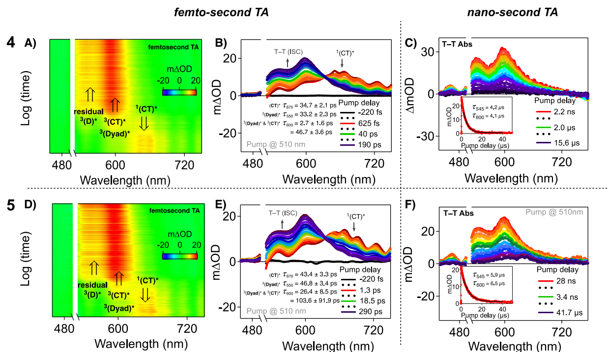
Fig. 5. Time-resolved transient absorption 2D intensity map/spectra for dyads 4 and 5 , and corresponding kinetics recorded in oxygen-free THF samples with optical density O.D. = 0.4 at \lambda_{\text{Exc}} = 510 nm. (A & B) fs-TA map/spectra for 4 ; (D & E) fs-TA map/spectra for 5 . (C) ns-TA spectra for 4 ; (F) ns-TA spectra for 5 . Pump power = 0.3 \mu\text{J}/\text{pulse} and 2.5 kHz repetition rate for fs-TA and 1 \mu\text{J}/\text{pulse} and 1 kHz repetition rate for ns-TA.
