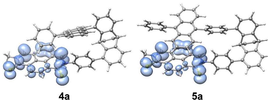
Fig. 4. Spin density at the T_1 optimized geometry of 4a and 5a optimized with CAM-B3LYP/6-31+G(d,p) in dichloromethane (surface isovalue = 0.002 a.u.).
