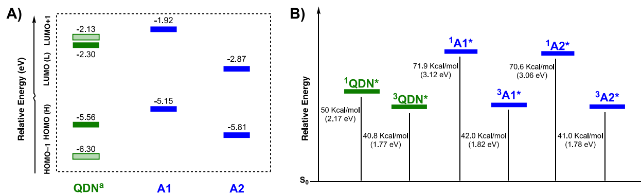
Fig. 6. (A) Optoelectronic bandgap of QDN a , A1, and A2. (B) singlet/triplet energy levels of QDN, A1, and A2. Note: QDN a represents QDN with one N -bromo-phenyl substituent.
