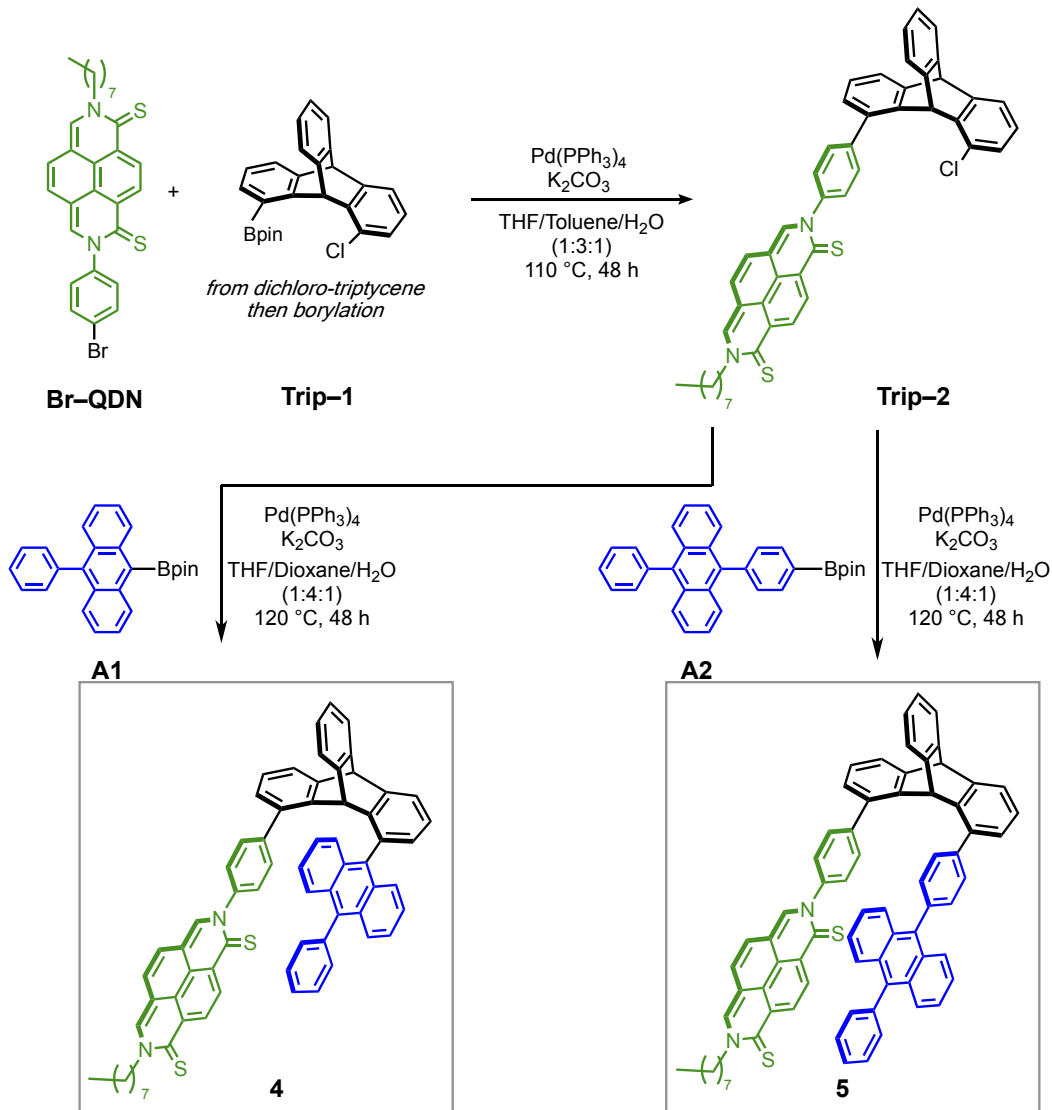
Scheme 1. Syntheses of triptycene-based D–A dyads 4 and 5 .
