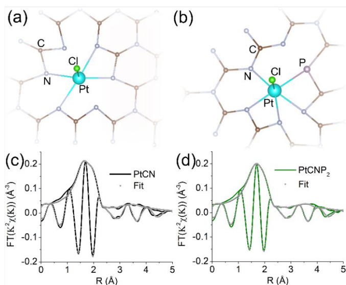
Figure 4. Ball and stick model representations of the fitting structures for (a) PtCN and (b) PtCNP 2 . Coordination to the centre Pt atom indicates first and second shell atoms used for fitting. Atoms are colour coded with carbon (brown), nitrogen (gray), platinum (cyan), chlorine (green), and phosphorous (light red). EXAFS fitting results shown in R-space for (c) PtCN and (d) PtCNP 2 . Raw R-space data is shown in solid with fits shown in gray circles. Fittings are performed in the R range of 1.3 to 2.5 Å.
