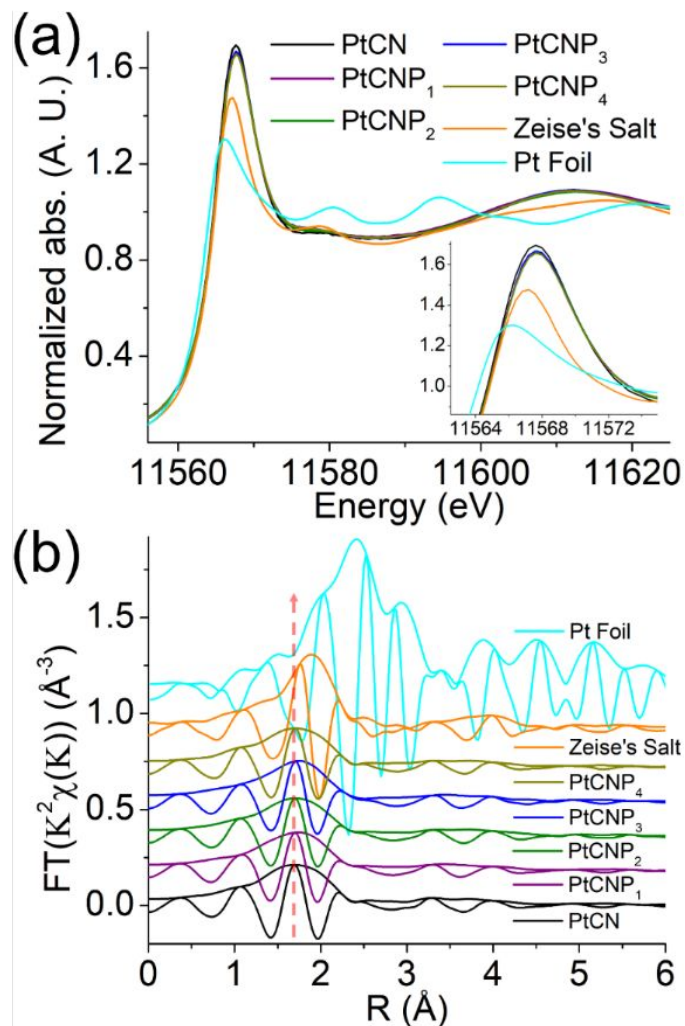
Figure 3. (a) Normalized Pt L3 edge XANES for the sample series in comparison to Pt Zeise's salt precursor (orange) and Pt foil (cyan). All edge steps are normalized to an edge height of 1. The energy range selected to normalize the edge is 11.7-12.0 keV. Measurements were performed at a temperature of 10K to reduce thermal disorder within samples. Inset is the zoom in of the white line region. (b) Pt L3 edge r-space EXAFS data for the sample series and two reference samples, Pt Zeise's salt (orange) and Pt Foil (cyan). The FT window is from 3.5 to 12.0 \text{ \AA}^{-1} , rounded using a Gaussian function of width, 0.2 \text{ \AA}^{-1} . The fast-oscillating function is the real part R of the FT, and the amplitude is (R^2+I^2)^{1/2} , whereas I is the imaginary part of the FT. Samples have been shifted vertically for better comparison.
