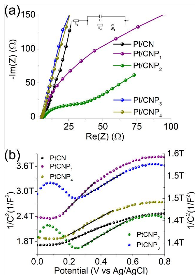
Figure 6. (a) Nyquist plots for the sample series produced from electrochemical impedance measurements at -10 mV overpotential. Inset is the Randle's equivalent circuit where R_1 is the solution resistance, R_{ct} is the charge-transfer resistance, C is the double-layer capacitance, and W_d is the Warburg diffusion term. (b) Mott-Schottky measurements for the sample series performed in 0.1 M Na_2SO_4 . Potentials are vs an Ag/AgCl reference electrode. Regression taken within the linear portion of each sample is shown as a black solid line. Y-axis on the left correspond to samples PtCN, PtCNP 1 , and PtCNP 3 while y-axis on the right corresponds to PtCNP 2 and PtCNP 4 .
