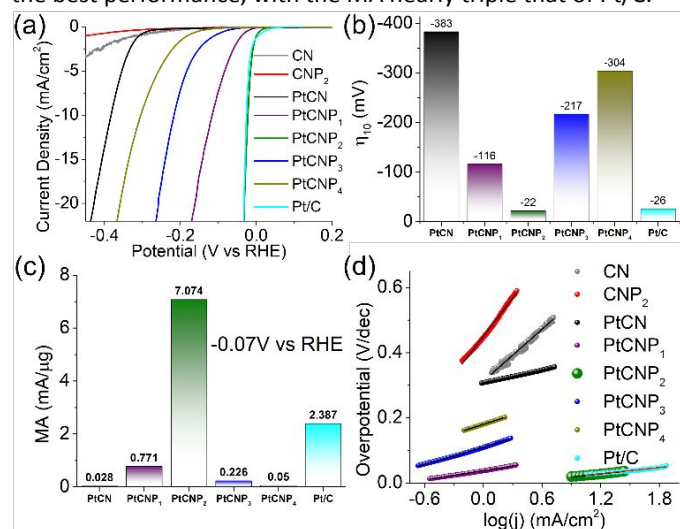
Figure 5. (a) HER polarization curves on various electrocatalysts in 0.5M H_2SO_4 at the rotation rate of 1600 rpm, potential sweep rate of 10 mV/s and 85% iR compensation. (b) Corresponding \eta_{10} from the HER polarization curves in panel (a). (c) Mass activity at -0.07 V vs RHE per \mu g of Pt calculated from ICP-OES measurements. (d) Tafel plots derived from panel (a). Note the overlapping data points between the Pt/C and PtCNP 2 samples.
