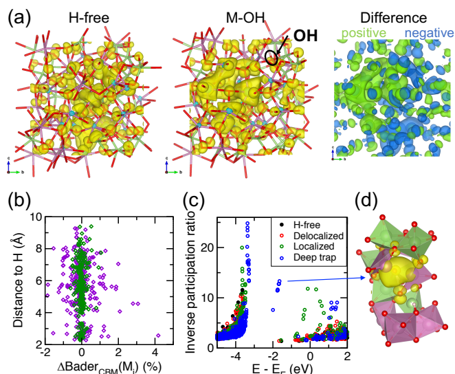
Fig. 7 (a) Charge density distribution in the conduction band for H-free a-In-Ga-O and H-doped a-In-Ga-O with M-OH defect with the lowest formation energy and the difference between the two charge density distributions showing the charge redistribution by the positive (green) and negative (blue) charge. (b) Difference in the Bader charge %-contributions to the bottom of the conduction band from individual metal atoms as a function of their distance from H defect in H-doped a-In-Ga-O. (c) Inverse participation ratio for the electronic states, see Eq. 2, in H-free and three cases for structures with M-OH defect resulting in delocalized conduction band (red), strongly localized states near the Fermi level (green), and deep trap states (blue). (d) The charge distribution between two under-coordinated In atoms surrounded by GaO polyhedra, resulting in the deep trap state shown in (c).
