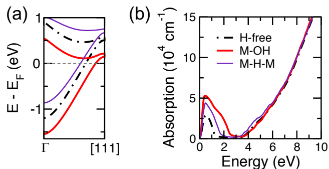
Fig. 8 (a) The electronic band-like structure calculated along [111] direction of the cubic cell for H-free a-In-Ga-O structure and the structures with M-OH and M-H-M defects having the lowest formation energies for each defect type. (b) Calculated optical absorption for the H-free and H-doped In-Ga-O as obtained from DFT-HSE calculations.
