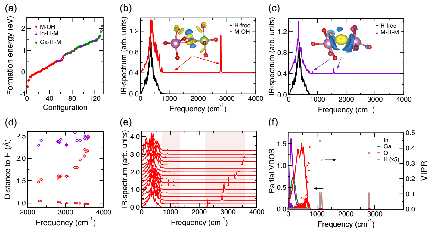
Fig. 3 (a) Calculated formation energy of optimized 134 configurations of H-doped a-In-Ga-O. The type of defect is determined by the type of the nearest neighbor of H (O, In, or Ga). (b) Calculated IR-spectrum for H-free a-In-Ga-O and the case with M-OH that has the lowest formation energy. The insert shows the calculated charge transfer for the HO bond with positive (yellow) and negative (blue) charge density distributions. (c) Calculated IR-spectrum for H-free a-In-Ga-O and H-doped case that corresponds to the M-H-M defect with lowest formation energy. The insert shows the calculated charge transfer for the In-H-In bond with positive (yellow) and negative (blue) charge density distributions. (d) IR-frequency of M-OH defects as a function of the H distance to its first and second nearest O neighbor (red cross and red diamond, respectively) and the nearest M neighbor (purple diamond). (e) Calculated IR-spectrum for representative H-doped a-In-Ga-O structures with M-OH defects. The shaded areas highlight the frequency ranges where peaks associated with the OH defect appear. (f) Calculated atom-resolved vibrational density of states (VDOS, solid lines) and vibrational inverse participation ratio (VIPR, circle markers) for the a-In-Ga-O case with M-OH that has the lowest formation energy.
