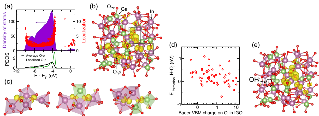
Fig. 2 (a) Total density of states (DOS) and state localization represented by inverse participation ratio in H-free a-In-Ga-O and partial DOS for oxygen p -states on average and for the O atom that shows the largest localization at the top of the valence band (VB). (b) The calculated total charge density distribution within the top VB in H-free a-In-Ga-O unit cell reveals several non-bonding O- p -orbitals with strong charge localization. Large purple (green) spheres represent In (Ga) atoms and small red spheres are O atoms. (c) Three pairs of dangling O- p -orbitals that give the largest charge contributions (boxed in (b)). The nearest neighbor metal polyhedra highlight the fact that the non-bonding O- p -orbitals are oriented by pointing away from a metal atom on either side of each orbital. (d) The calculated formation energy of the structures with M-OH defect is plotted as a function of the Bader charge contribution from the oxygen in the OH defect to the top of VB in H-free a-In-Ga-O. (e) Charge density distribution within the top of VB reveals passivation of one of the dangling O- p -orbital pair in the structure with the lowest formation energy.
