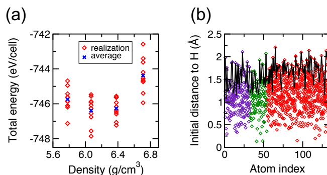
Fig. 1 (a) Calculated total energy of amorphous In-Ga-O as a function of cell density. Ten independent MD realizations (liquid quench followed by equilibration) for each density were performed. (b) 1,000 “trial” positions for H atom are represented by the distance from H to its nearest neighbor In (purple), Ga (green), or O (red) atom. The black line connects the longest distances at which the given atom remains to be the nearest neighbor of H. In each of the 134 initial configurations, a single interstitial H radical was placed near one of the 134 atoms at this longest distance from the given atom.
