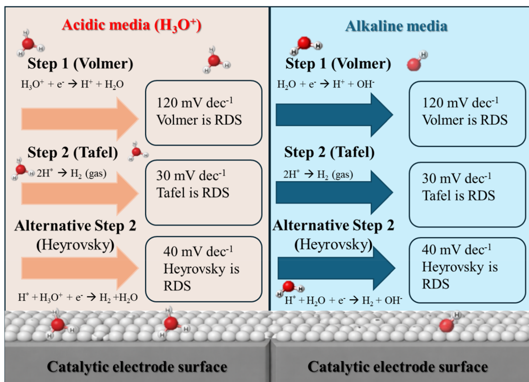
Fig. 2 Comparison of HER mechanisms and theoretical Tafel slopes.
