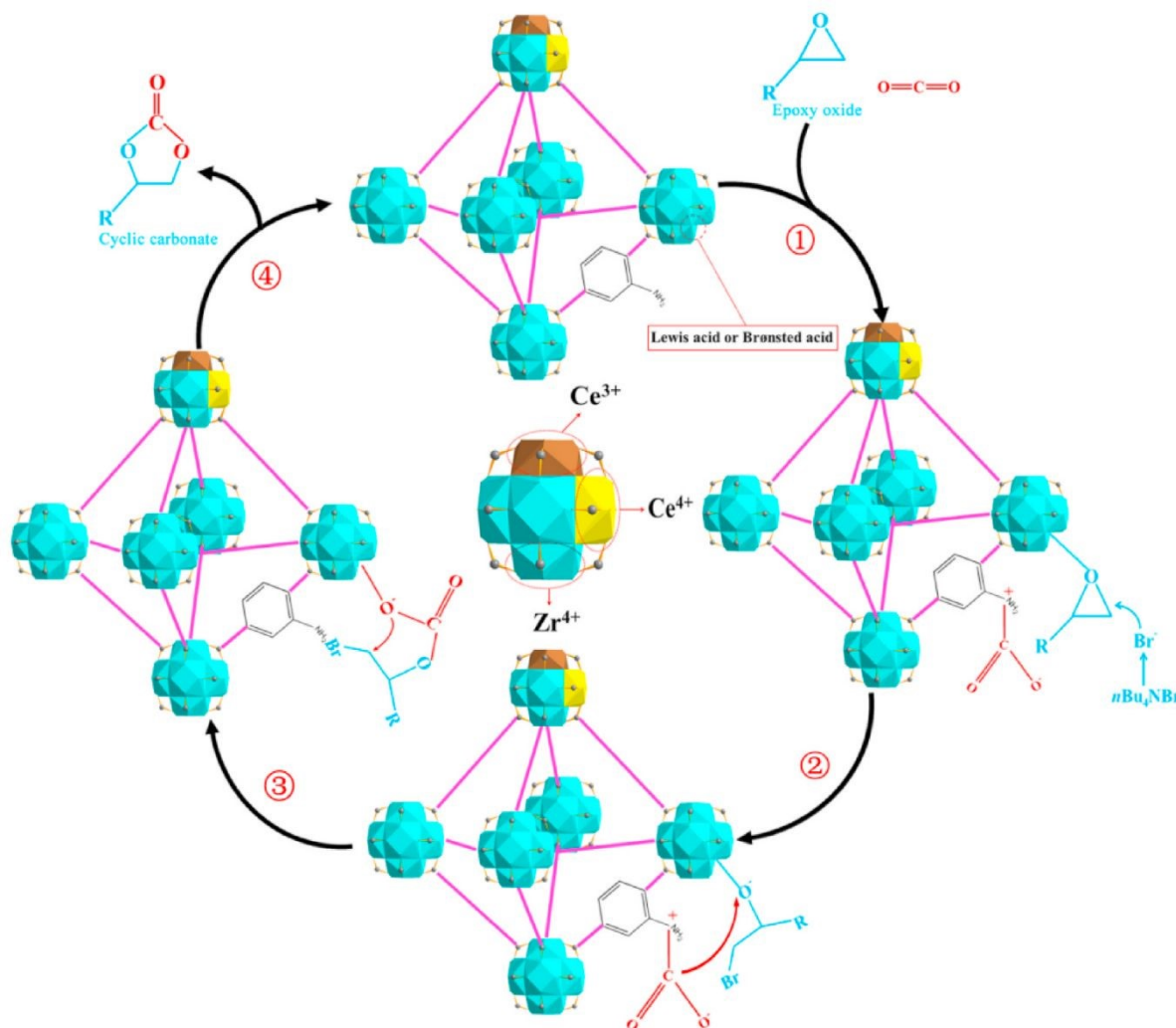
Figure 16. Proposed mechanism for the cycloaddition of \text{CO}_2 and epoxides by defective bimetallic UiO-66- \text{NH}_2(\text{Zr/Ce}) catalyst. 1) Through the catalyst, epoxy oxide is integrated with Lewis or Brønsted acid sites and is activated. Due to the presence of the -\text{NH}_2 group on MOF, \text{CO}_2 is adsorbed and polarized; 2) The nucleophilic \text{Br}^- ion attacks the \beta carbon atom of epoxide to form the Oxygen anion intermediate; 3) The intermediate interacts with \text{CO}_2 to create halogenated carbonate; 4) Through internal cyclization, halogenated carbonate is converted into cyclic carbonate, meanwhile the catalyst is regenerated. Reproduced with permission from ref. 293 Copyright 2021 Elsevier.
