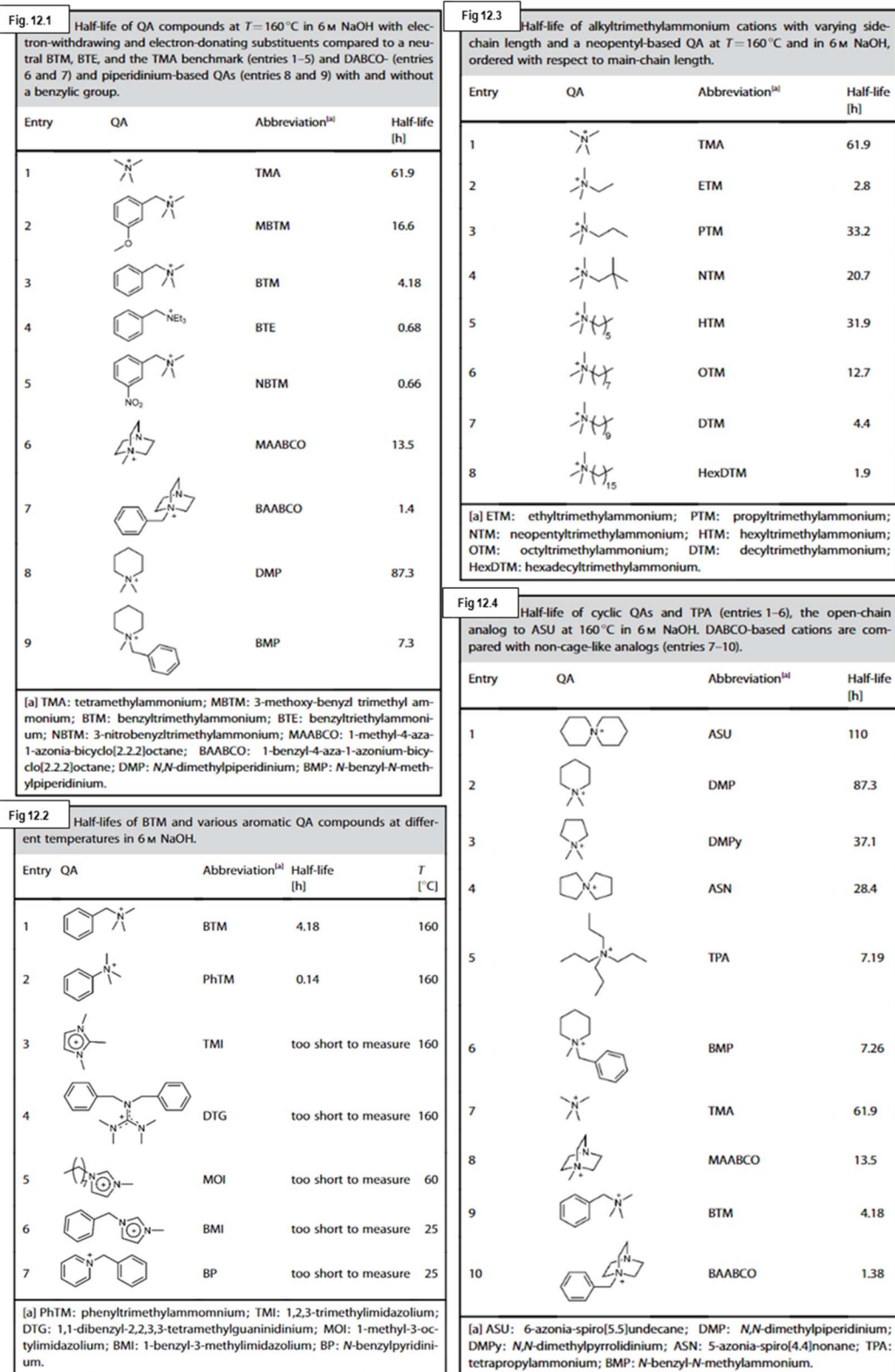
Fig. 12 Alkaline stability of the most common cationic groups given as half-life values. Adapted from Marino and Kreuer 76 with permission from John Wiley and Sons (License N° 5917551209635).
