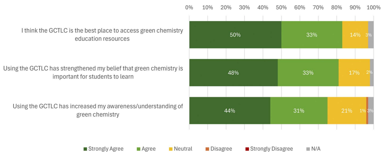
Fig. 3 Belief of respondents that the GCTL is the best place to access green chemistry education resources, and that using the GCTL has increased respondents' awareness/understanding of green chemistry and strengthened their belief that green chemistry is important for students to learn.
