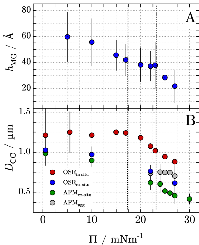
Fig. 7 (A) The first moment ( h_{MG} ) of the slabs j = 1, 2 that represent the parts of the MG that protrude into the air superphase above the apparent air/water interface ( z \geq 0 Å), as calculated from the SLD profiles presented in Fig. 5. (B) Centre-to-centre distances ( D_{CC} ) of MG particles deduced with OSR at the air/water interface ( in situ ) and with AFM and OSR on Langmuir–Blodgett transferred samples ( ex situ ) as a function of lateral pressure \Pi .
