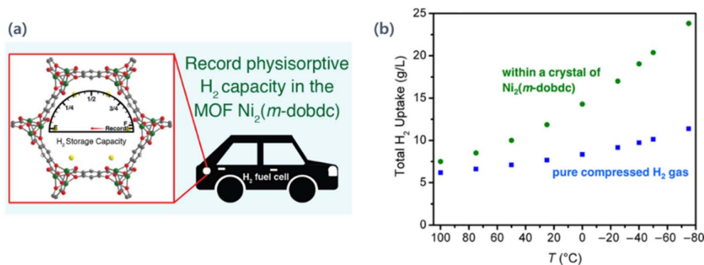
Fig. 9 (a) Schematic illustration of the physisorptive H 2 capacity in \text{Ni}_2(\text{m-dobdc}) and (b) comparison of total volumetric capacities and pure compressed H 2 of \text{Ni}_2(\text{m-dobdc}) at 100 bar 147 (reproduced from ref. 147 with permission from The American Chemical Society, copyright 2018).
