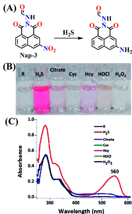
Fig. 3 (A) Chemical structure of Nap-3 and its corresponding amino product formed upon reduction by H_2S . (B) Naked eye image of H_2S selectivity among all RSS and ROS by Nap-3 (labelled as R) via colorimetric output. (C) Electronic absorption response of receptor Nap-3 with all RSS and ROS. Reproduced with permission from ref. 58. Copyright 2020, Royal Society of Chemistry.
