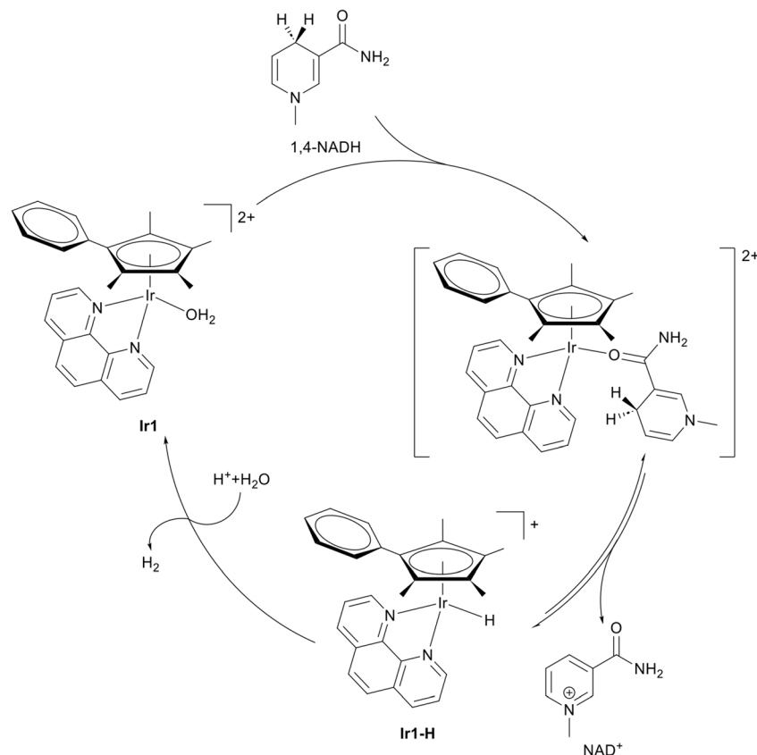
Fig. 6 Chemical structure of [(\eta^5\text{-C}_5\text{Me}_4\text{C}_6\text{H}_5)\text{Ir}(\text{phen})(\text{H}_2\text{O})]^{2+} (Ir1) and its catalytic conversion of NADH to \text{NAD}^+ by hydride transfer.
