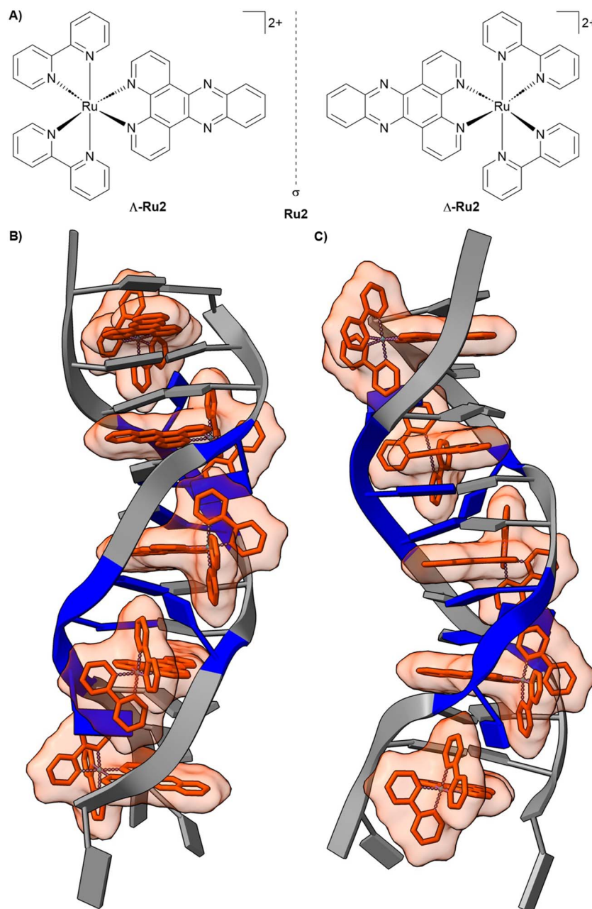
Fig. 3 Representative metal complex as a DNA binder. (A) Chemical structure of the racemic mixture of [Ru(bpy)_2(dppz)]^{2+} (Ru2), showing the \Delta -Ru2 and \Lambda -Ru2 enantiomers. (B) Front view of \Delta - [Ru(bpy)_2(dppz)]^{2+} ( \Delta -Ru2) bound to the oligonucleotide 5'-C 1 G 2 G 3 A 4 A 5 A 6 T 7 T 8 A 9 C 10 C 11 G 12 -3' (PDB: 4E1U). (C) 90° rotated view around the helix axis. Data originally reported by ref. 107 (H. Song et al. , 2012).
